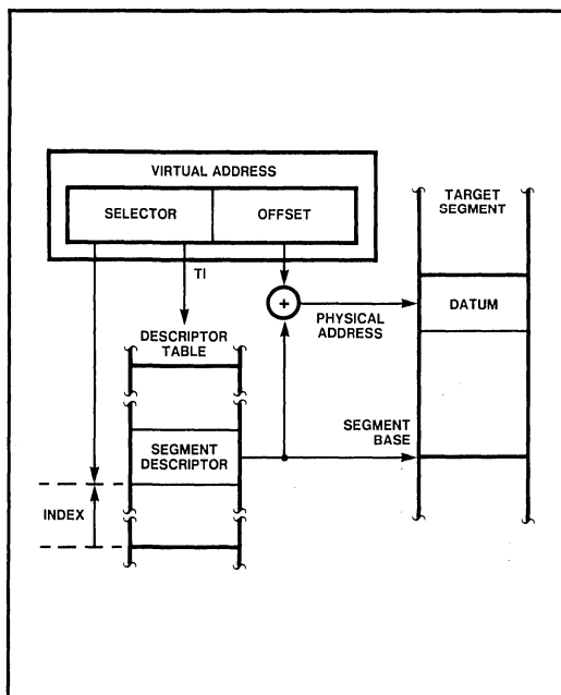
Figure 6-6. Virtual-to-Physical Address Translation
