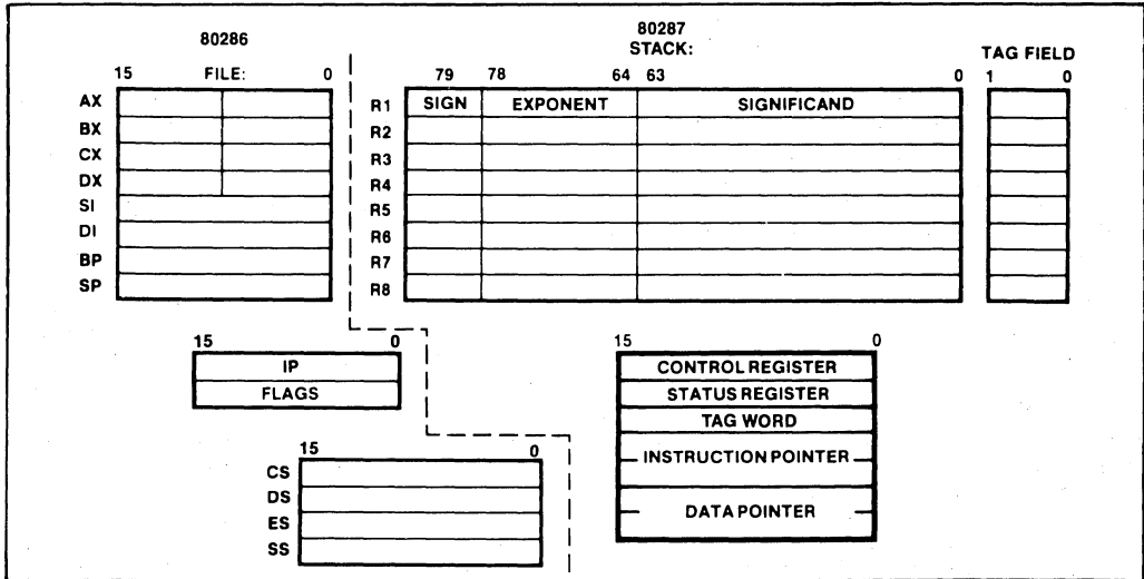
Figure 3. iAPX 286/20 Architecture
