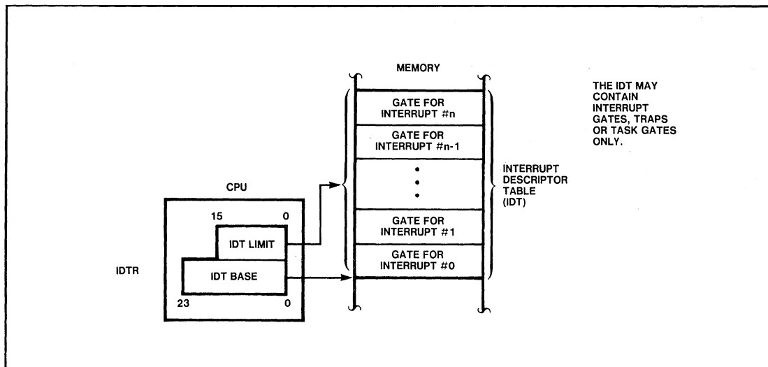
Figure 9-1. Interrupt Descriptor Table Definition
