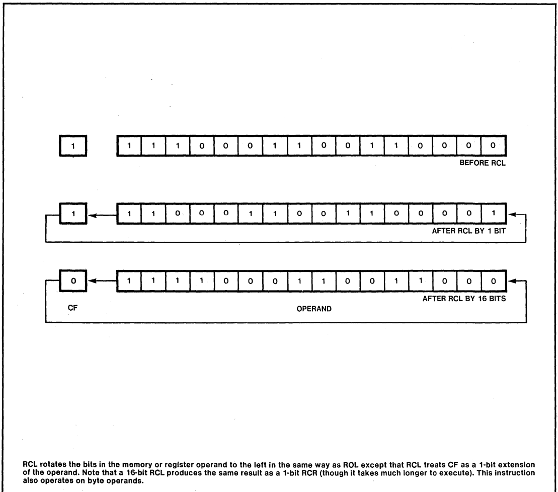
Figure 3-11. RCL
