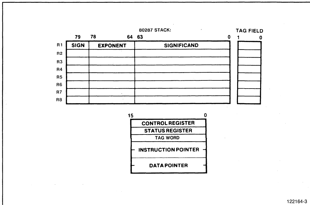
Figure 1-3. 80287 Register Set
