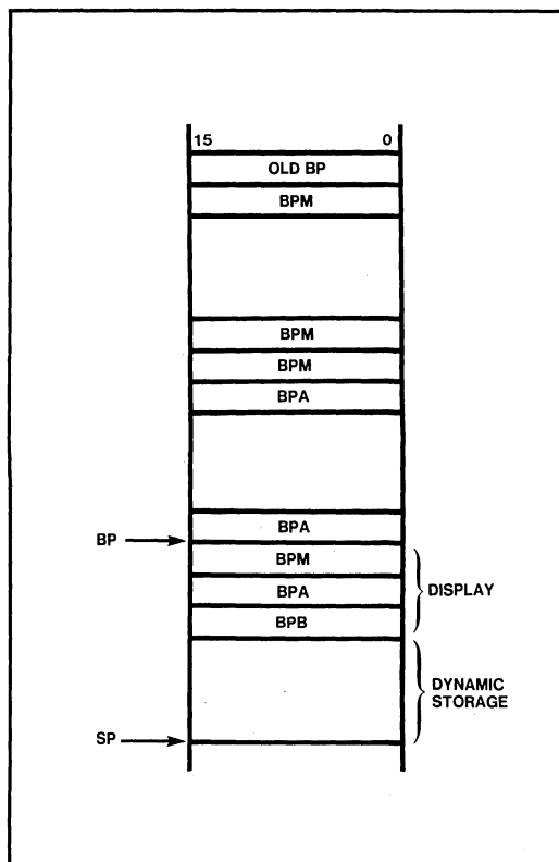
Figure 4-2c. Stack Frame for Procedure B at Level 3 Called from A
