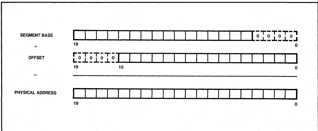
Figure 5-1b. Forming the 20-Bit Physical Address in the Real Address Mode
