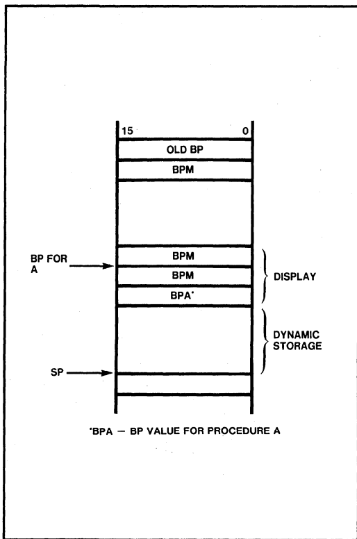
Figure 4-2b. Stack Frame for Procedure A
