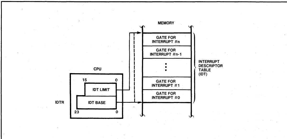
Figure 10-2. Interrupt Descriptor Table Definition
