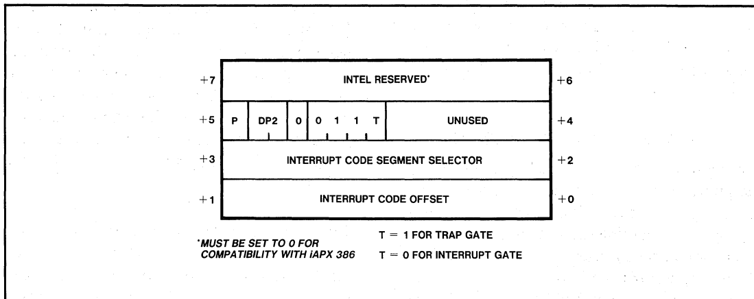
Figure 9-3. Trap/Interrupt Gate Descriptors
