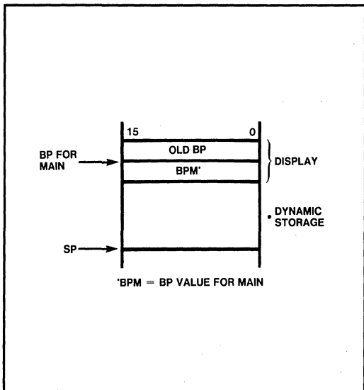
Figure 4-2a. Stack Frame for MAIN at Level 1
