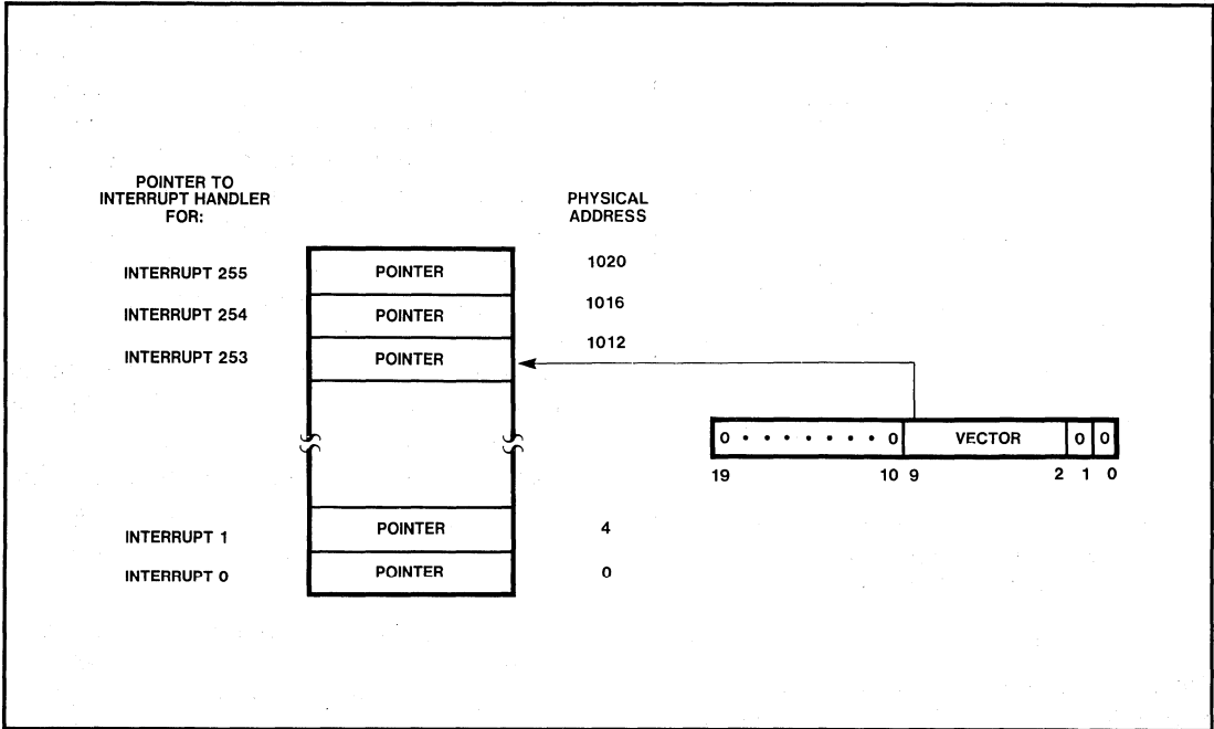
Figure 5-3. Interrupt Vector Table for Real Address Mode
