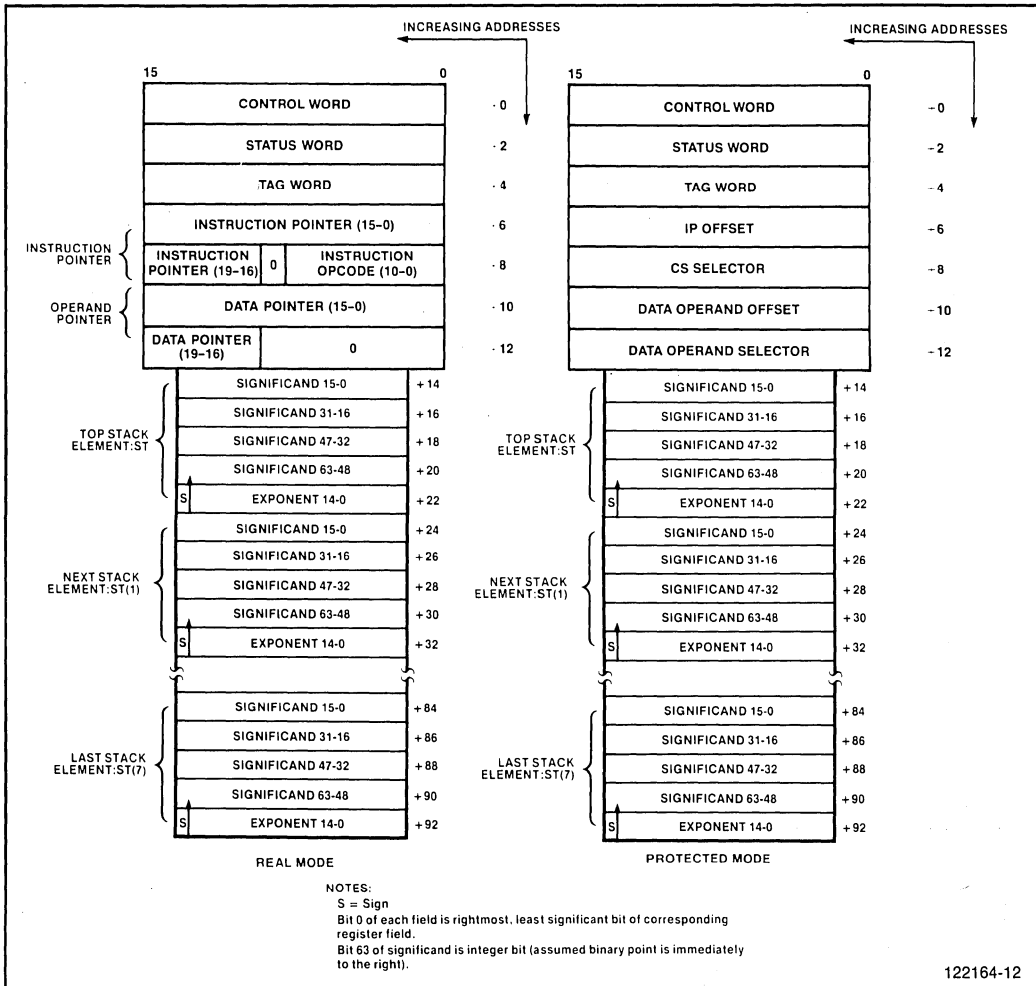
Figure 2-1. FSAVE/FRSTOR Memory Layout
