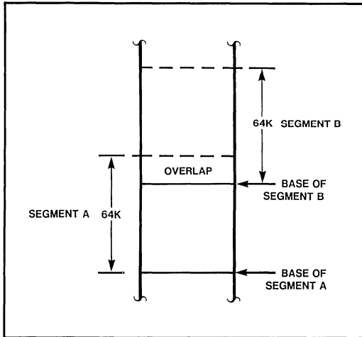
Figure 5-2. Overlapping Segments to Save Physical Memory
