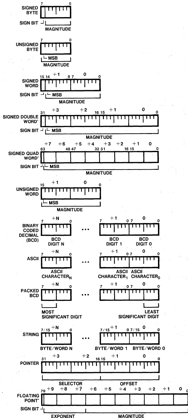
Figure 2-3. IAPX 286 Supported Data Types
