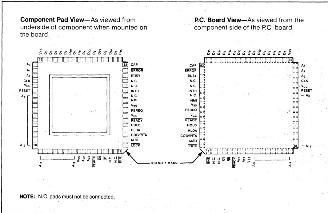
Figure 2. 80286 Pin Configuration
