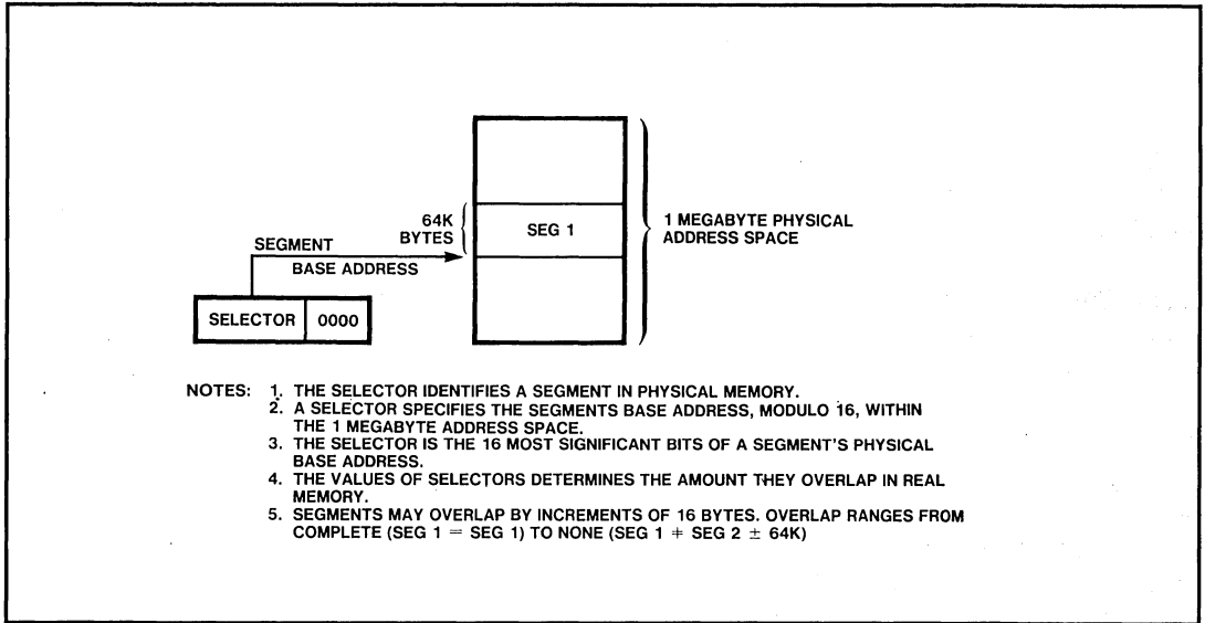
Figure 2-5. Real Address Mode Segment Selector Interpretation
