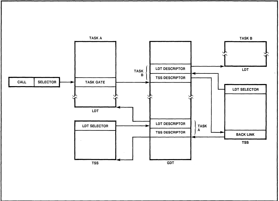
Figure 8-4. Task Switch Through a Task Gate
