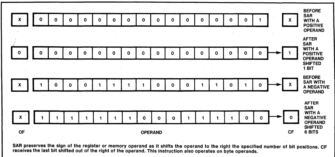
Figure 3-8. SAR
