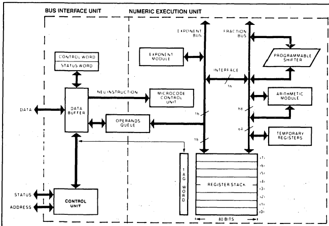
Figure 1. 80287 Block Diagram
