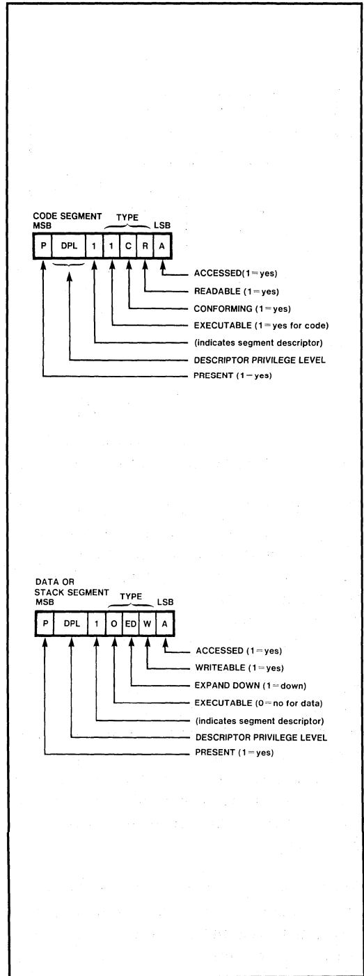
Figure 6-7. Segment Descriptor Access Bytes
