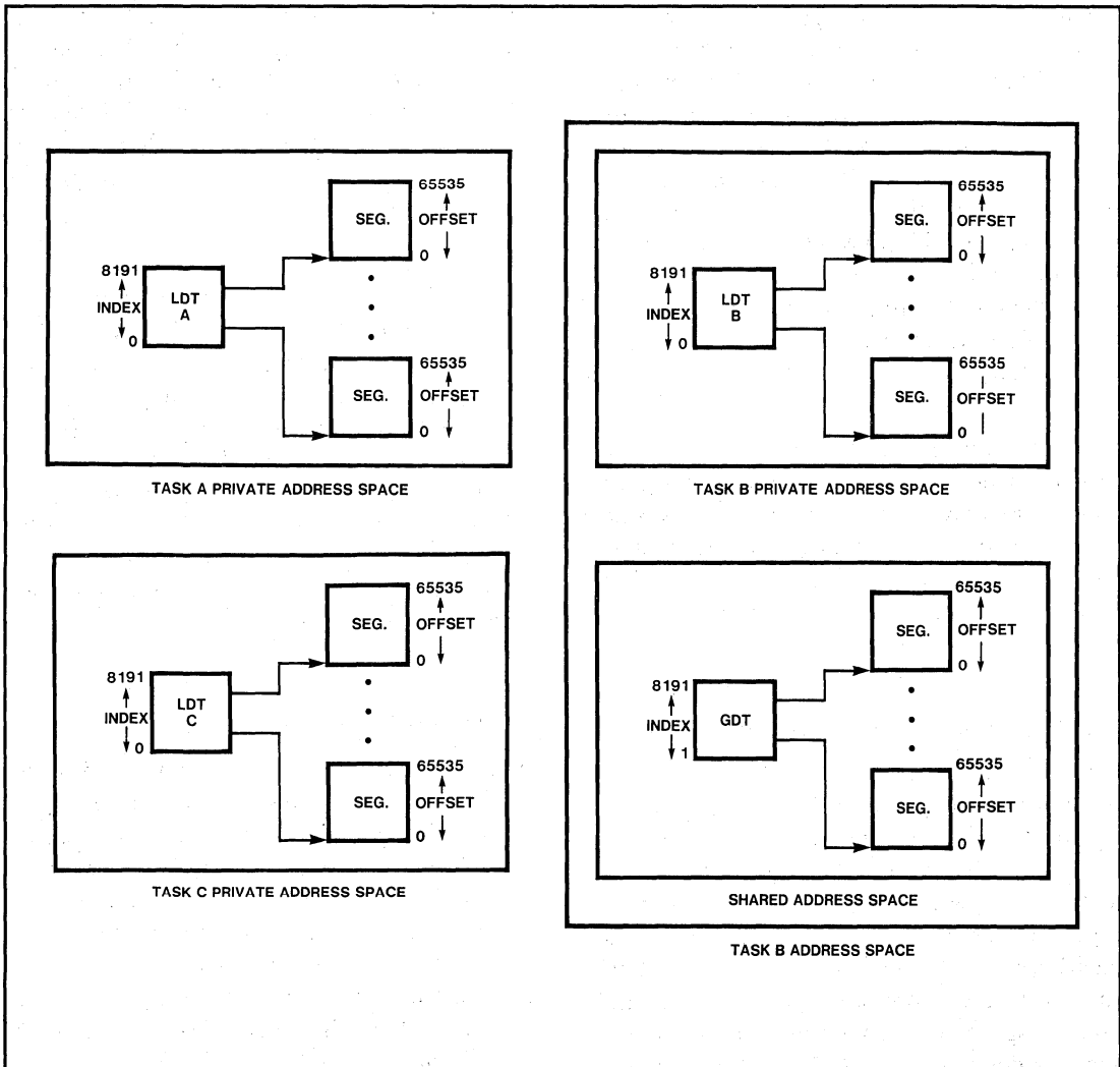
Figure 7-3. IAPX 286 Virtual Address Space
