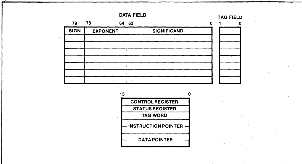
Figure 5. 80287 Register Set
