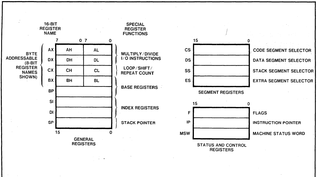
Figure 2-4. IAPX 286 Base Architecture Register Set
