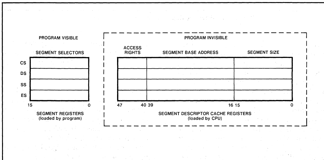
Figure 7-2. Descriptor Cache Registers
