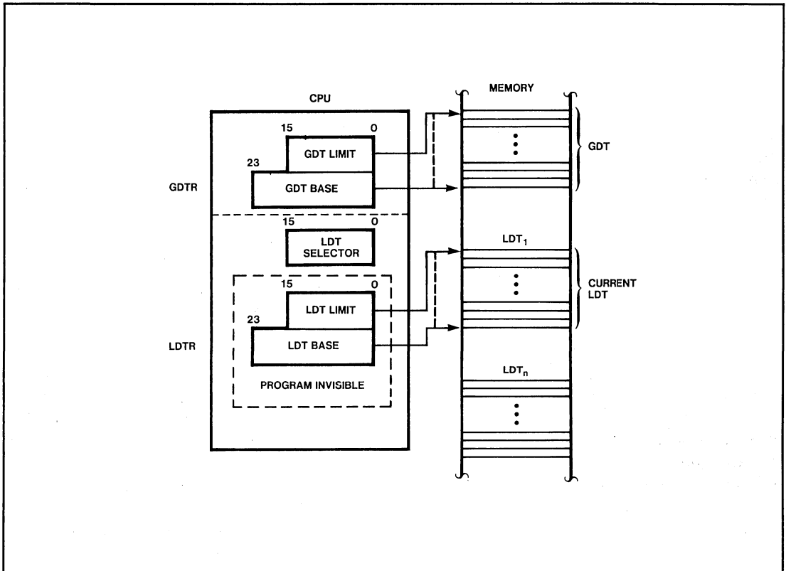
Figure 7-4. Local and Global Descriptor Table Definition
