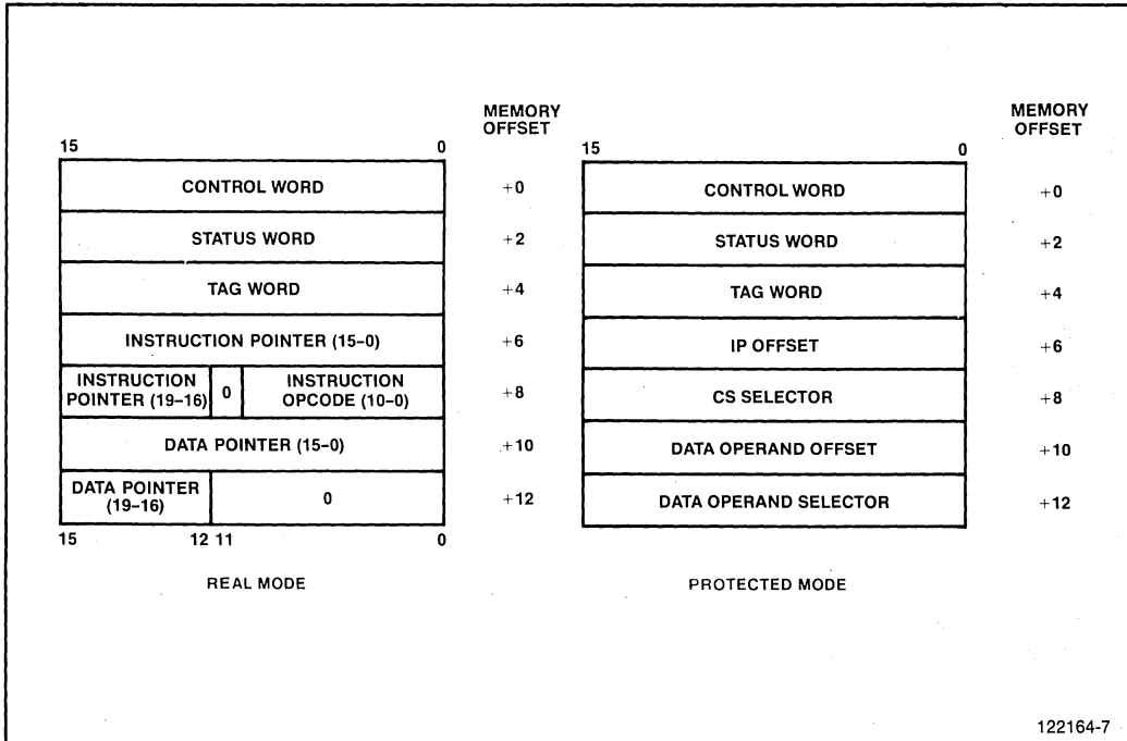
Figure 1-7. 80287 Instruction and Data Pointer Image in Memory
