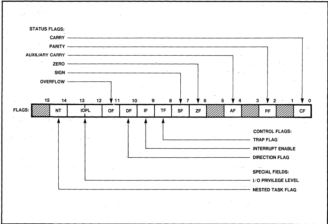
Figure 3-5. Flag Word Contents
