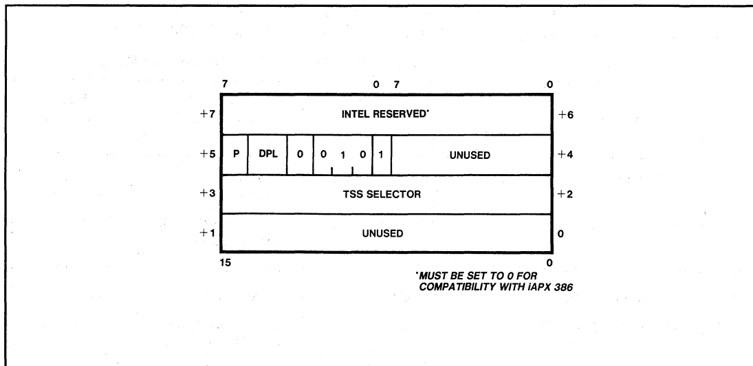
Figure 8-3. Task Gate Descriptor
