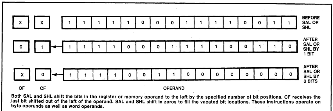
Figure 3-6. SAL and SHL
