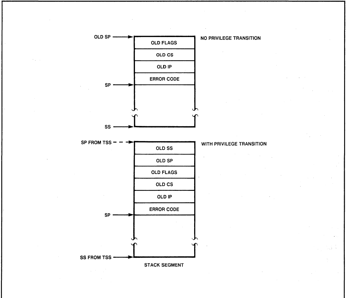
Figure 9-4. Stack Layout After an Exception with an Error Code
