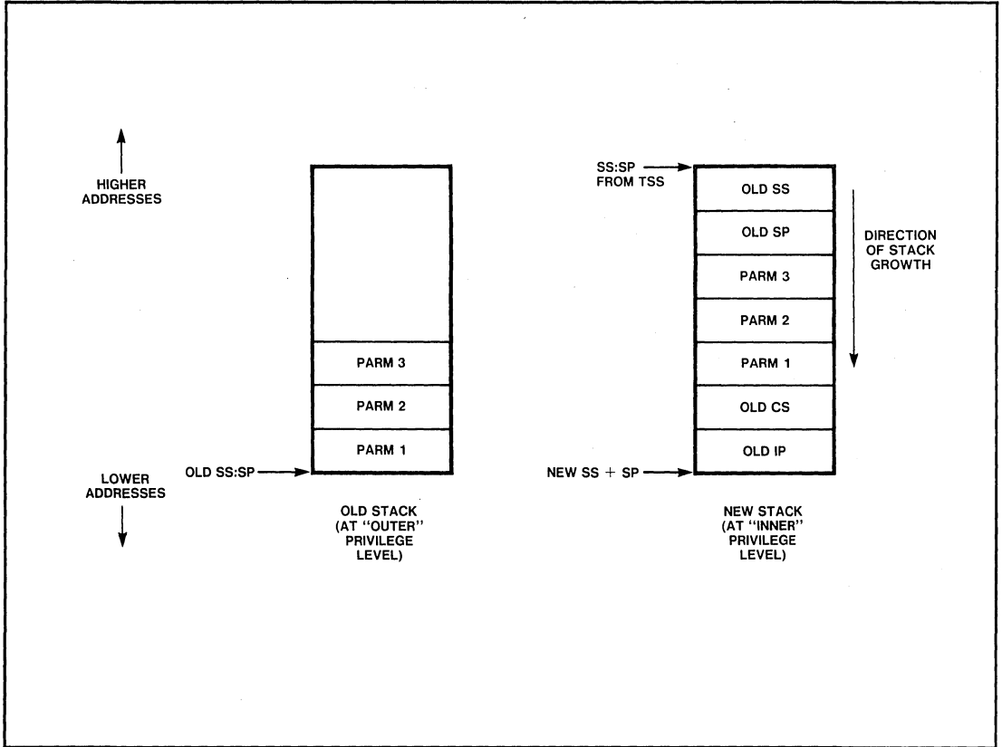
Figure 7-12. Stack Contents After an Inter-Level Call
