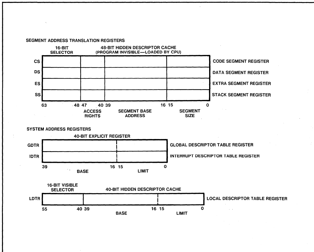
Figure 6-8. Memory Management Registers
