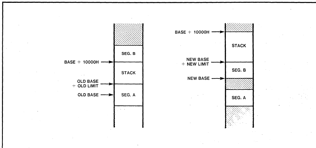
Figure 11-2. Dynamic Segment Relocation and Expansion of Segment Limit
