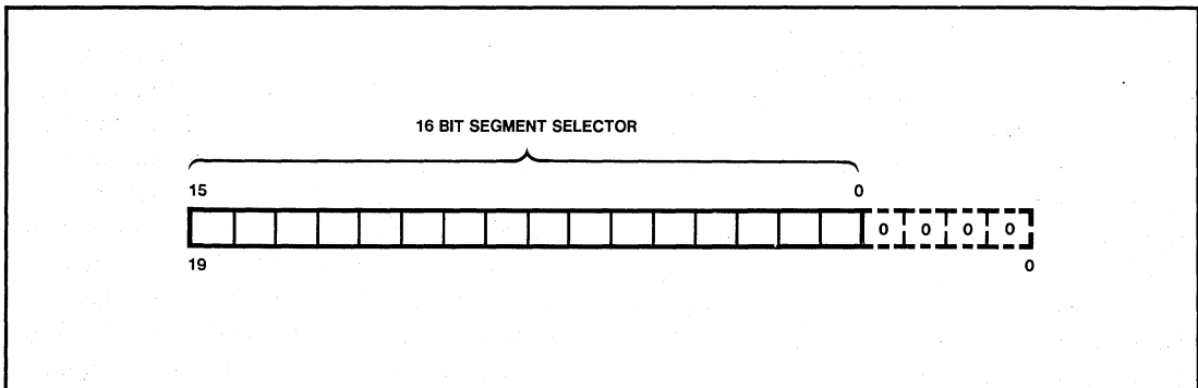
Figure 5-1a. Forming the Segment Base Address
