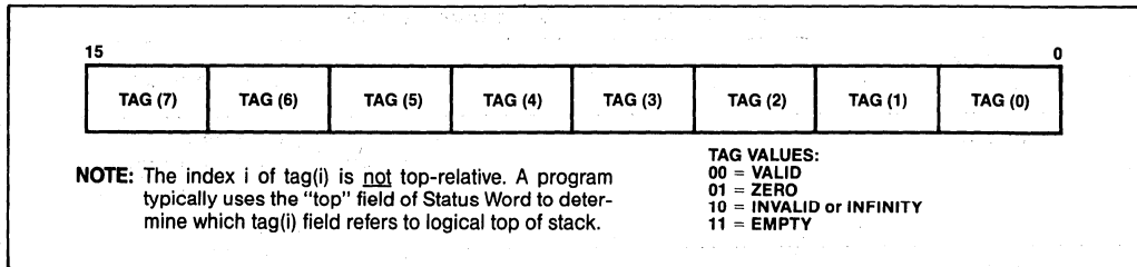
Figure 7. 80287 Tag Word
