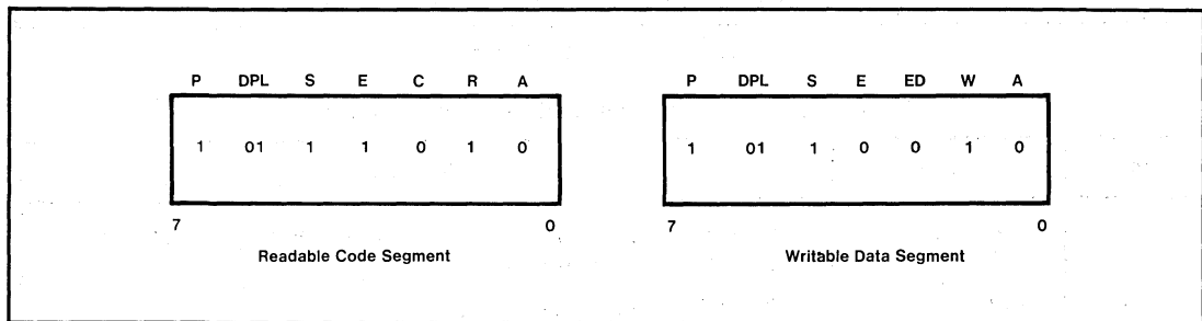
Figure 7-8. Access Byte Example
