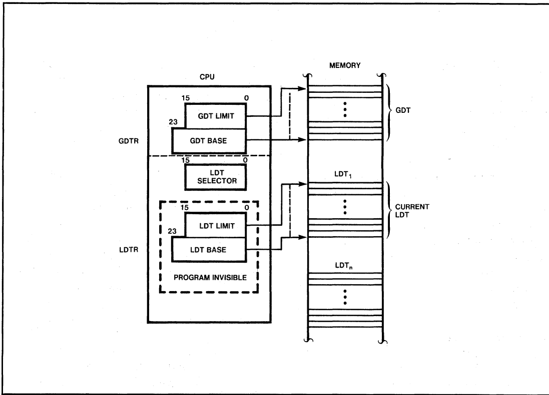
Figure 10-1. Local and Global Descriptor Table Definition
