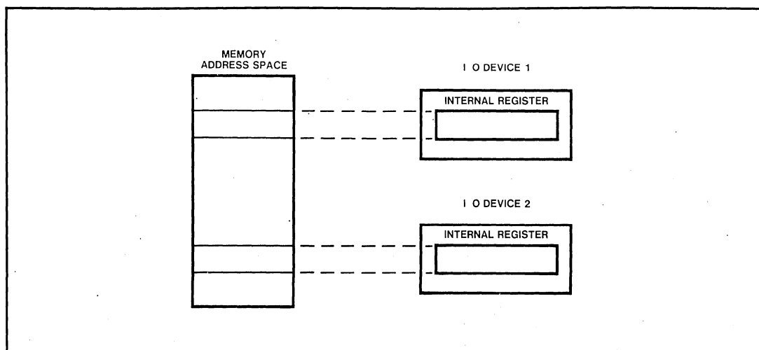
Figure 2-14. Memory-Mapped I/O
