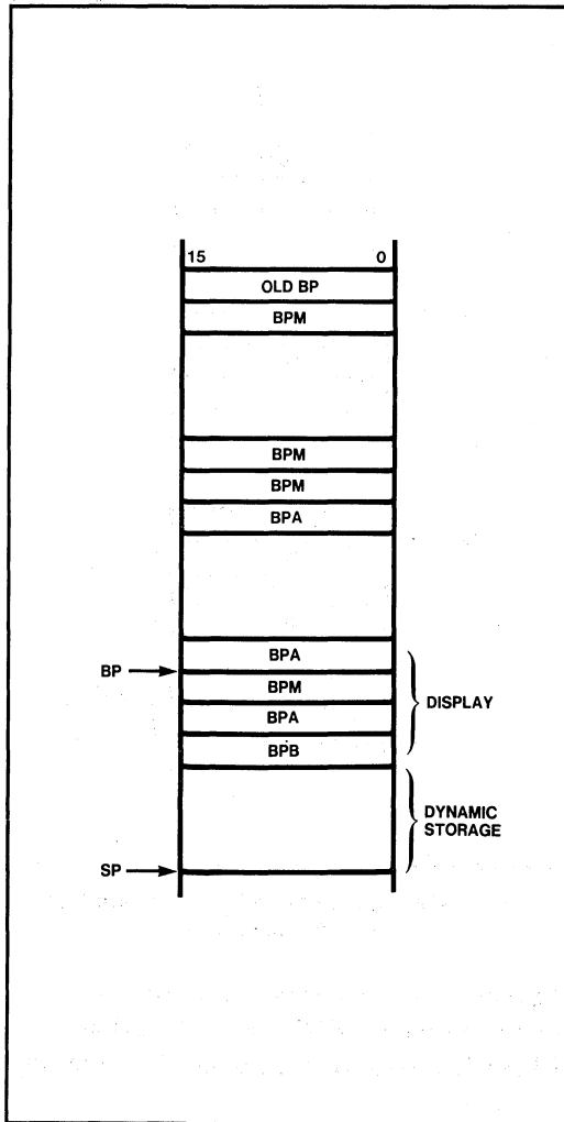
Figure 4-2d. Stack Frame for Procedure C at Level 3 Called from B
