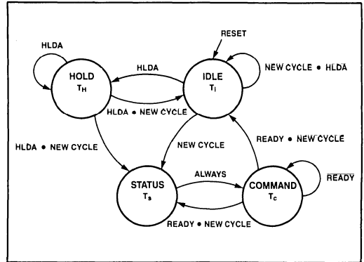
Figure 22. 80286 Bus States
