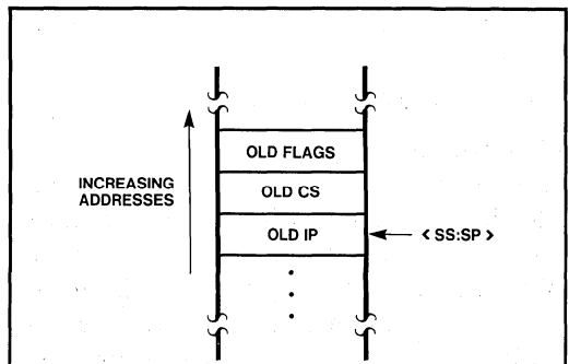
Figure 5-4. Stack Structure After Interrupt (Real Address Mode)
