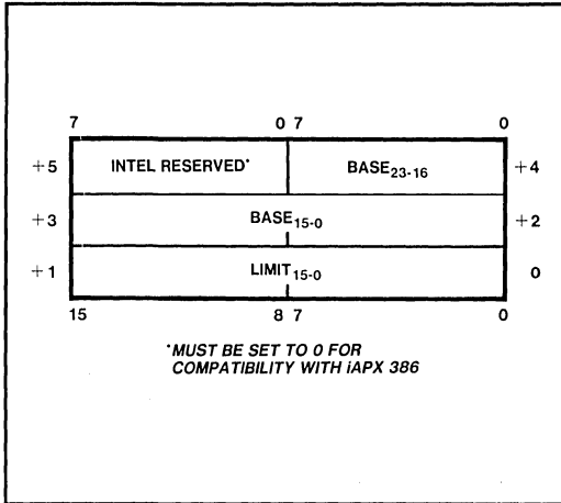
Figure 10-3. Data Type for Global Descriptor Table and Interrupt Descriptor Table
