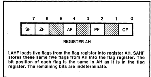
Figure 3-13. LAHF and SAHF
