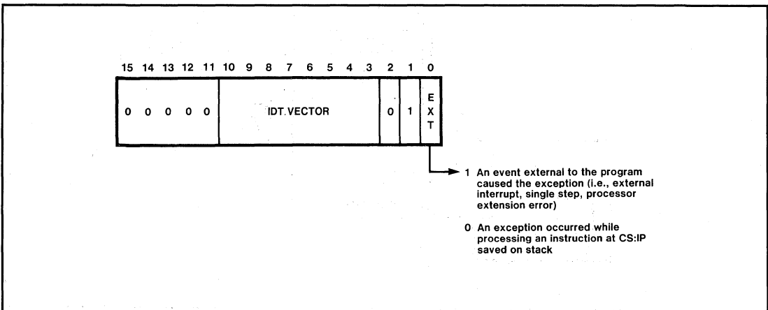
Figure 9-2. IDT Selector Error Code
