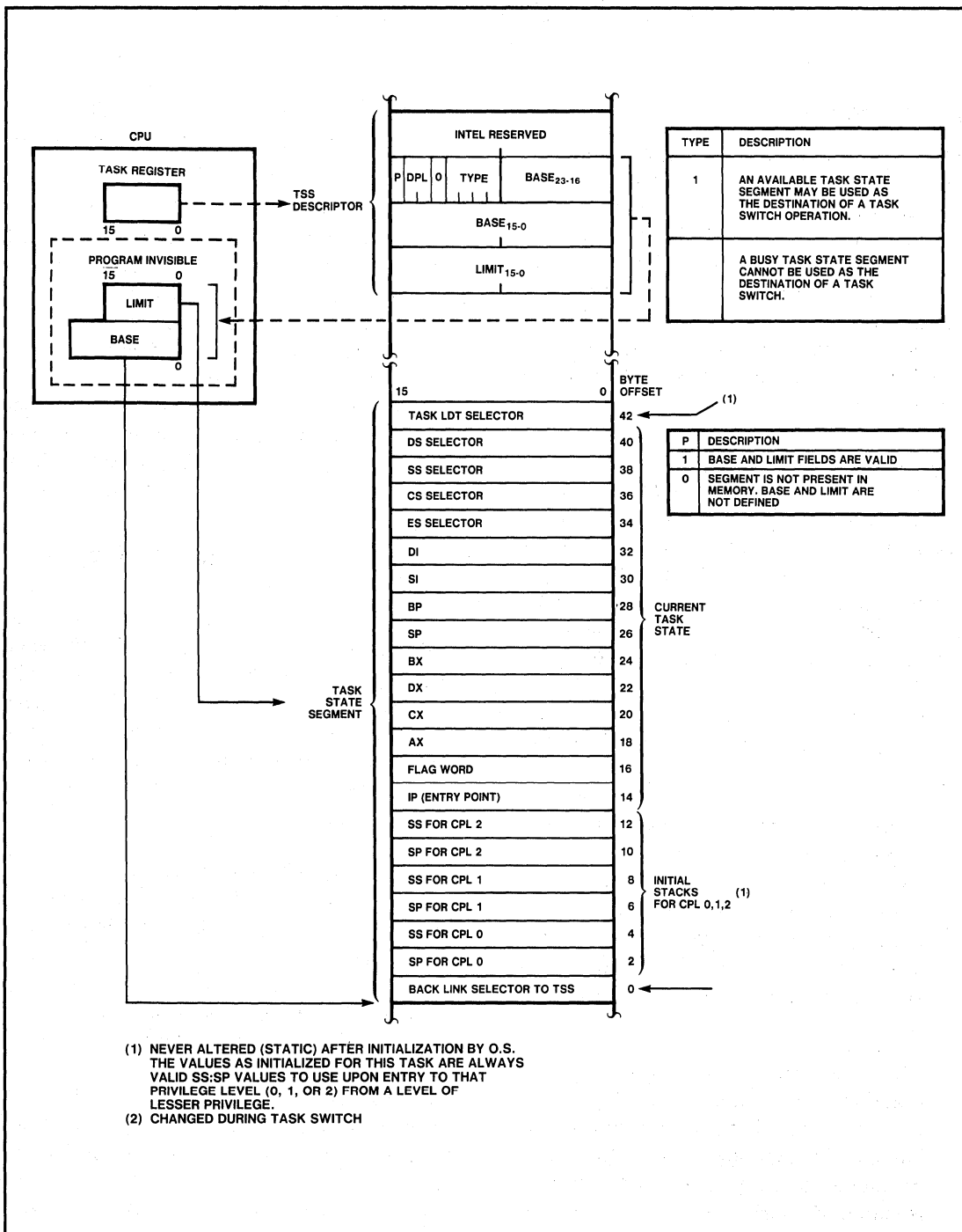
Figure 8-1. Task State Segment and TSS Registers
