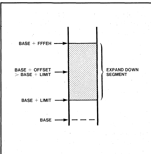
Figure 11-1. Expand-Down Segment
