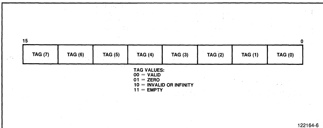
Figure 1-6. 80287 Tag Word Format
