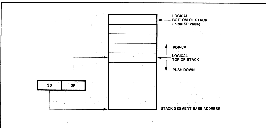
Figure 2-7. iAPX 286 Stack
