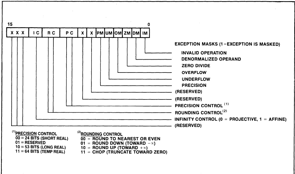
Figure 9. 80287 Control Word
