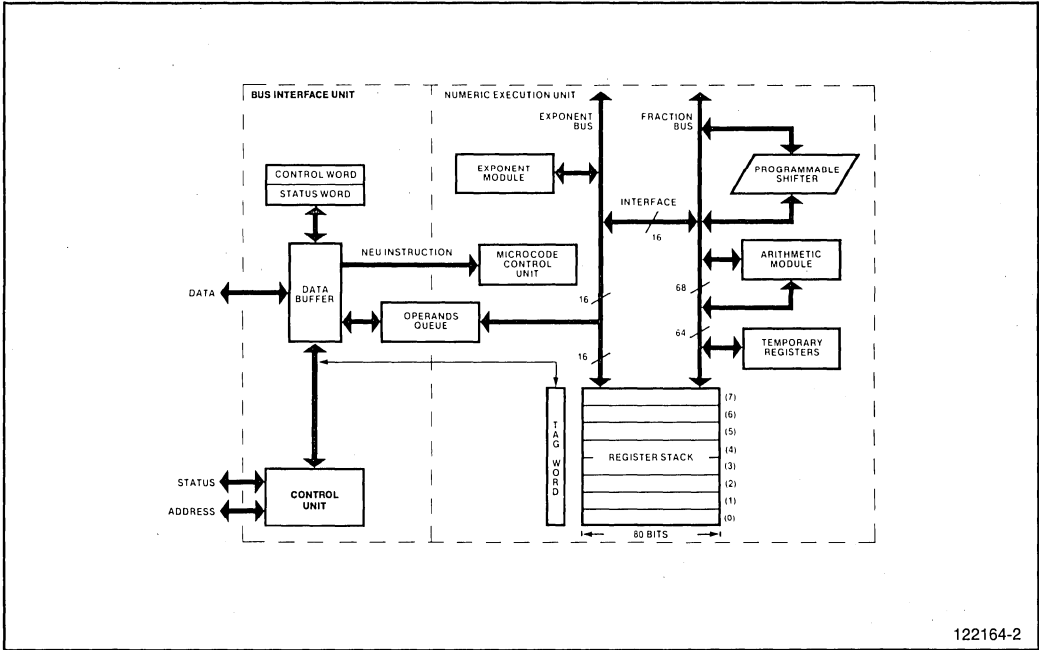
Figure 1-2. 80287 NPX Block Diagram
