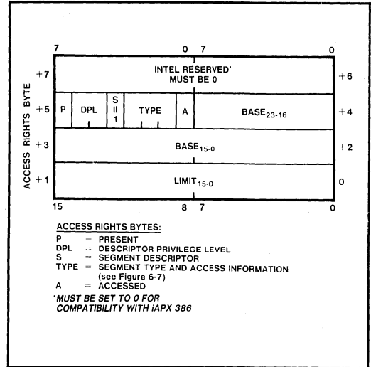
Figure 6-3. Segment Descriptor (S = 1)
