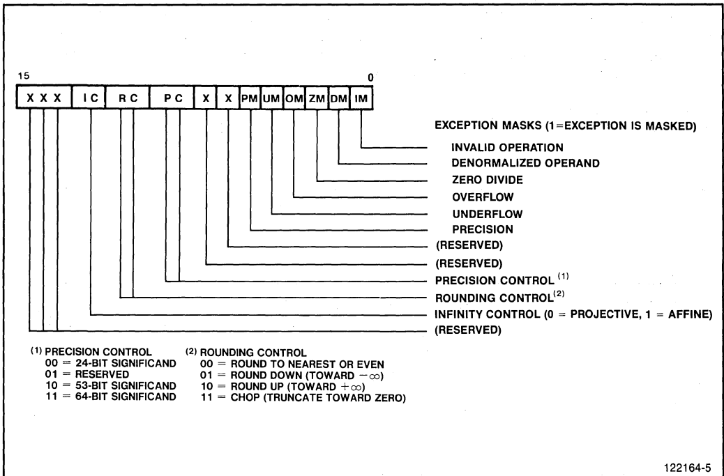
Figure 1-5. 80287 Control Word Format
