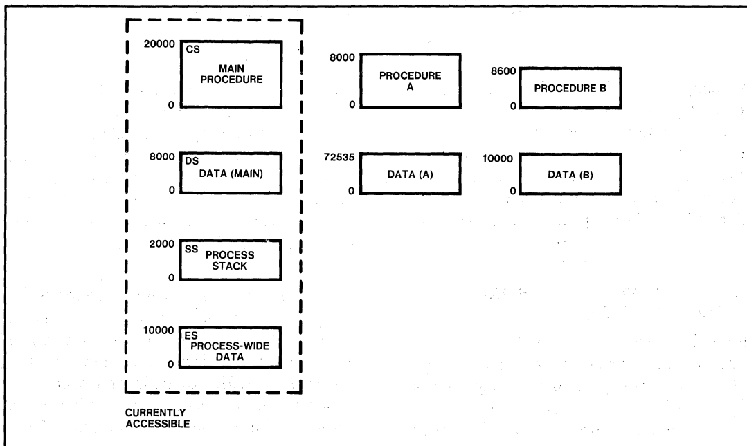
Figure 2-1. Segmented Virtual Memory
