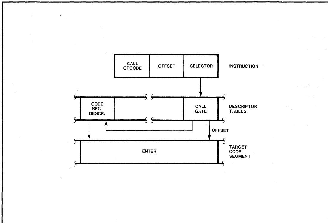
Figure 7-11. Call Gate
