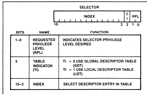
Figure 15. Selector Fields
