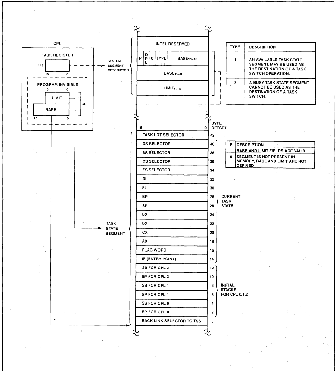
Figure 20. Task State Segment and TSS Registers
