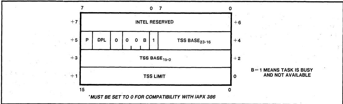
Figure 8-2. TSS Descriptor
