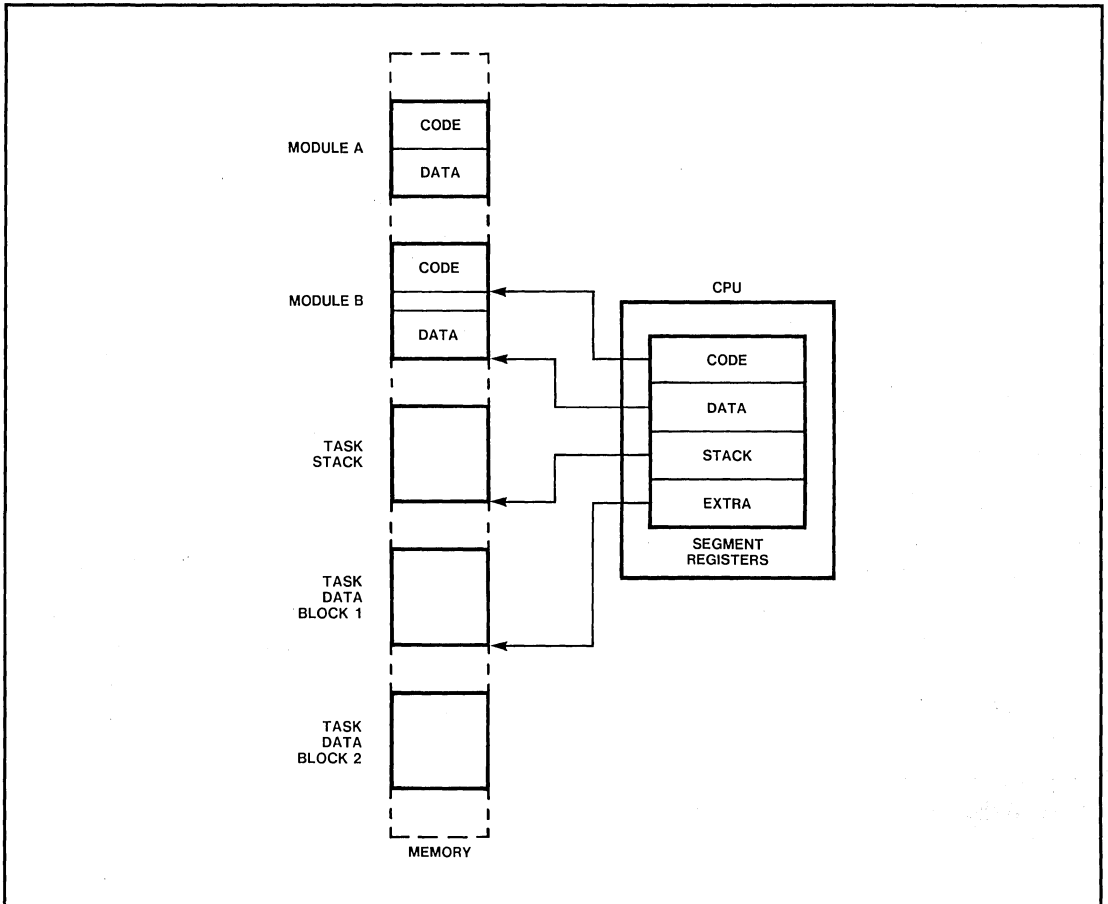
Figure 7-1. Addressing Segments of a Module Within a Task
