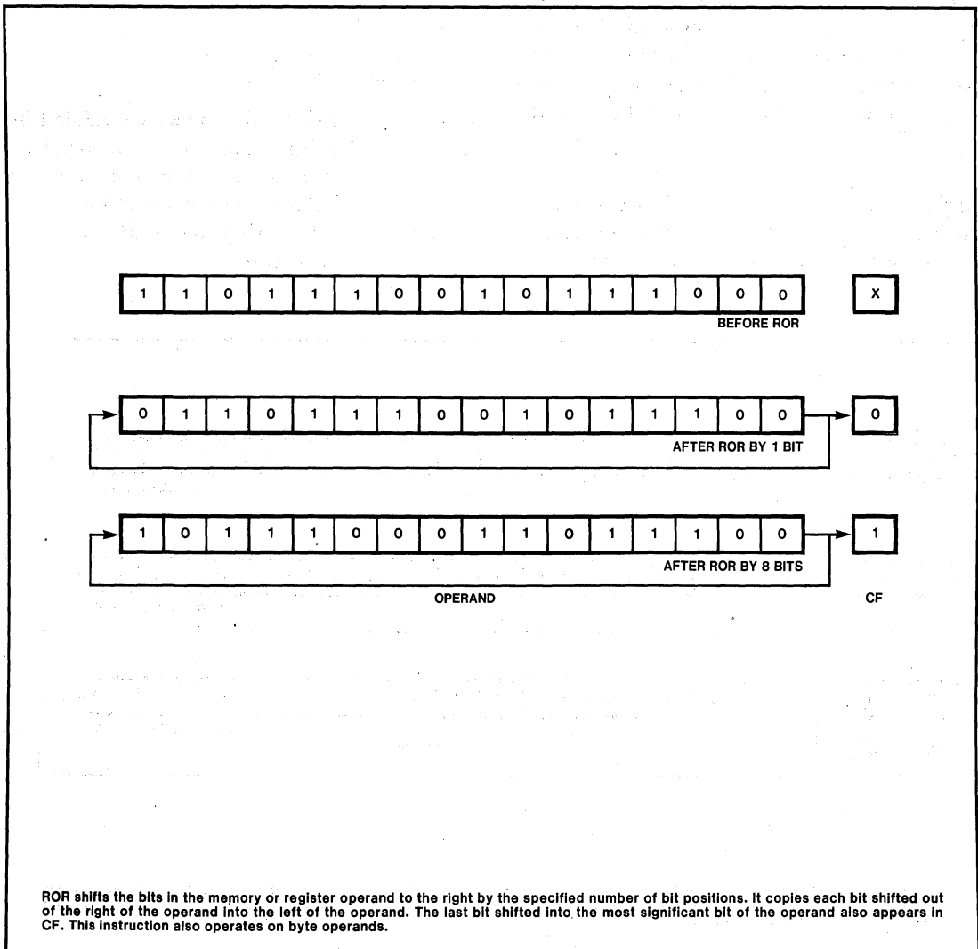
Figure 3-10. ROR
