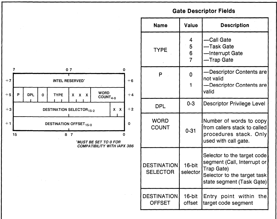
Figure 7-10. Gate Descriptor Format
