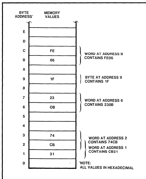
Figure 2-2. Bytes and Words in Memory
