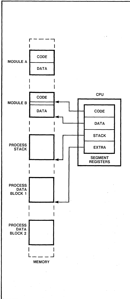
Figure 2-12. Use of Memory Segmentation
