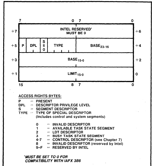
Figure 6-4. Special Purpose Descriptors or System Segment Descriptors (S = 0)
