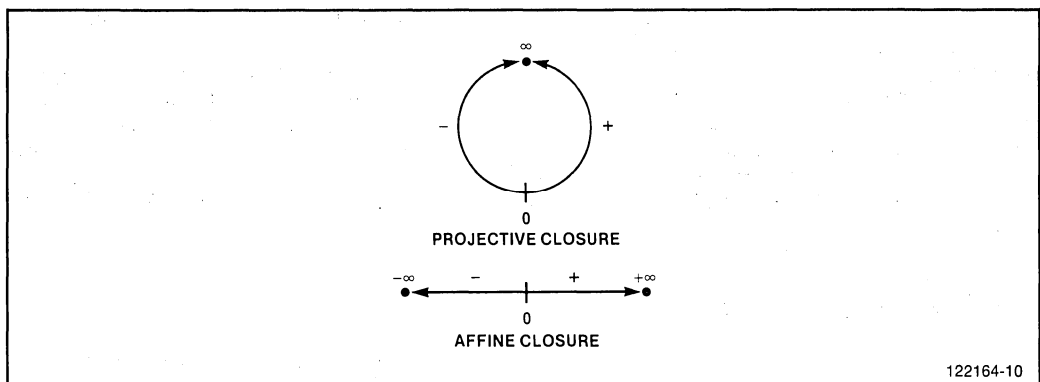
Figure 1-10. Projective versus Affine Closure
