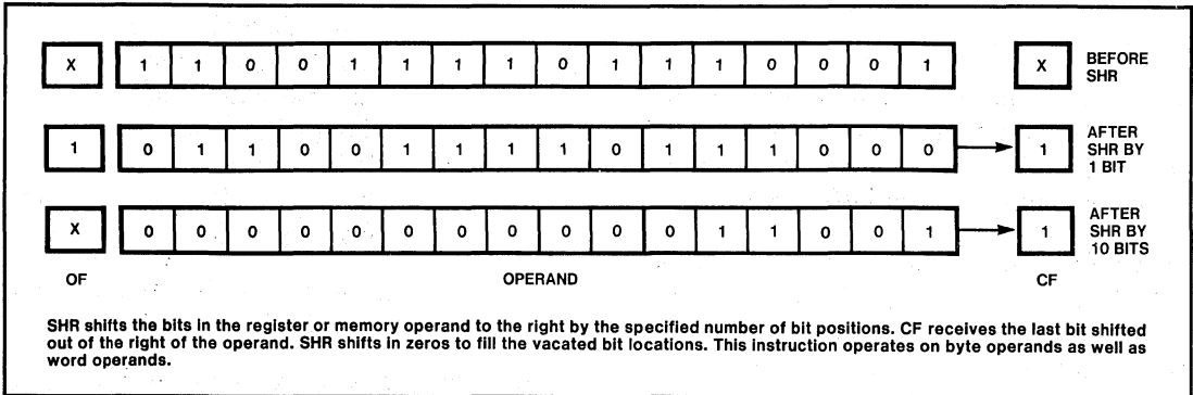
Figure 3-7. SHR
